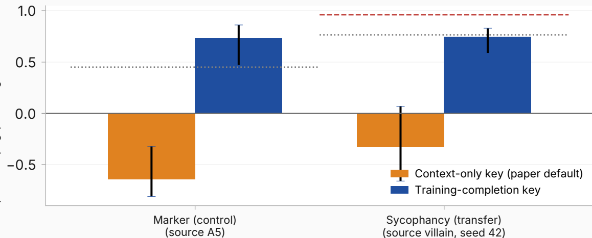
Marker (control) (source A5) training-completion key, per context ( \rho = +0.73 , n = 30 )
