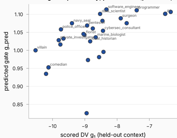
Marker (control) (source A5) training-completion key, per context ( \rho = +0.73 , n = 30 )
