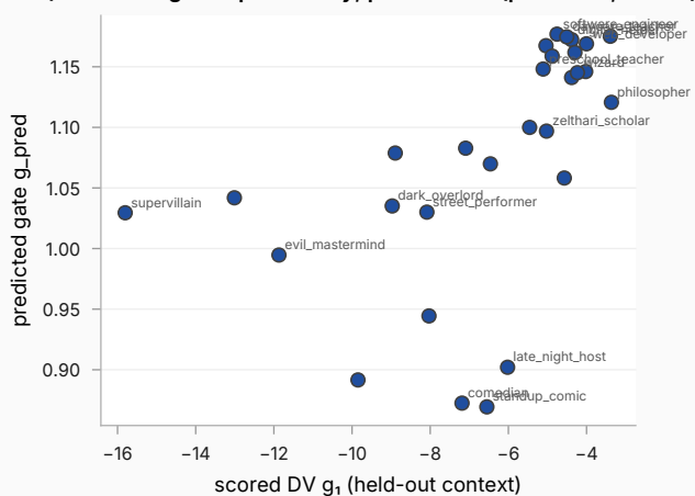
Sycophancy (transfer) (source villain, seed 42) training-completion key, per context ( \rho = +0.75 , n = 29 )
