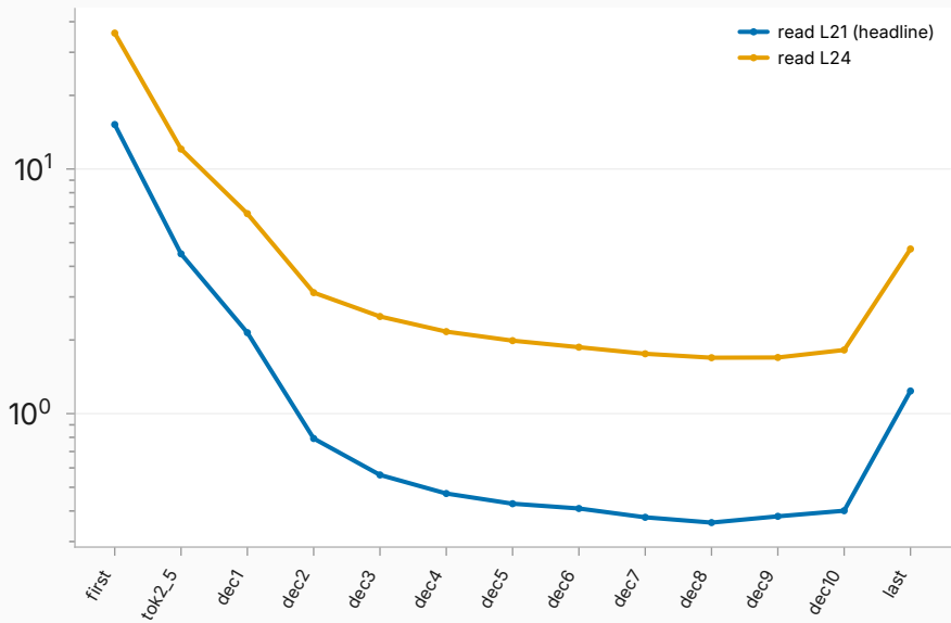
direct magnitude by read layer — baseline_text/L20
