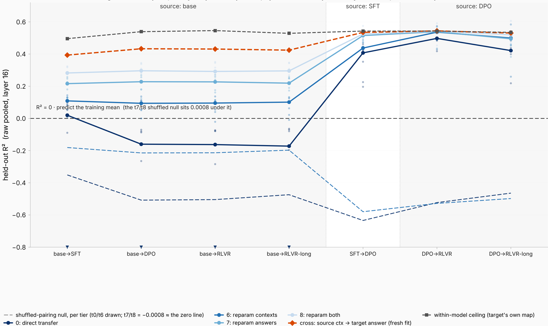
Every forward pair of the Tülu-3 ladder: how much of the context→answer map survives median over 7 non-degenerate corpora, every corpus overplotted; open markers = point-only (round B, no bootstrap draws)
