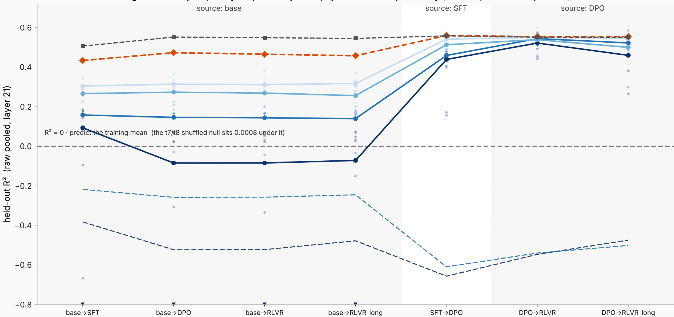
Every forward pair of the Tülu-3 ladder: how much of the context→answer map survives median over 7 non-degenerate corpora, every corpus overplotted; open markers = point-only (round B, no bootstrap draws)
