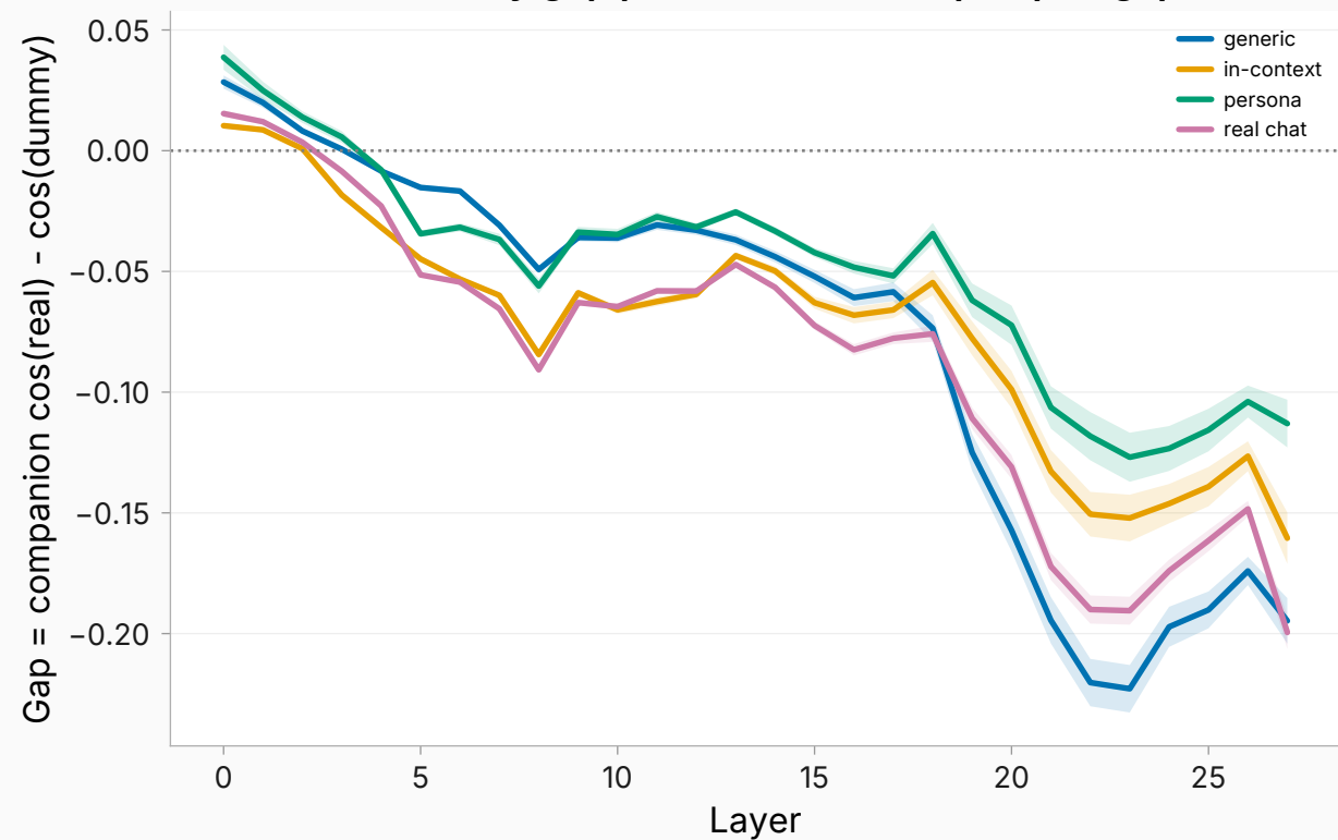
Real-minus-dummy gap per tier (shaded = per-pair gap SE)
