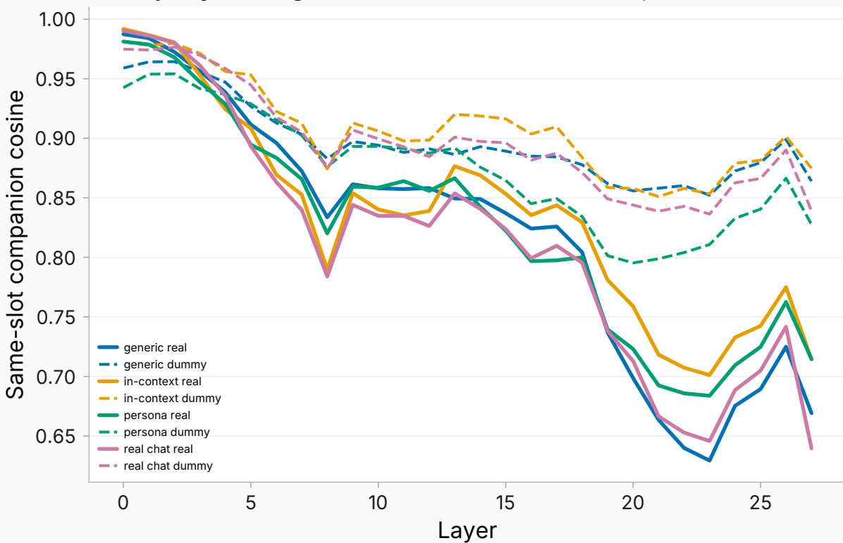
Real query vs length-matched no-content filler, same slot
