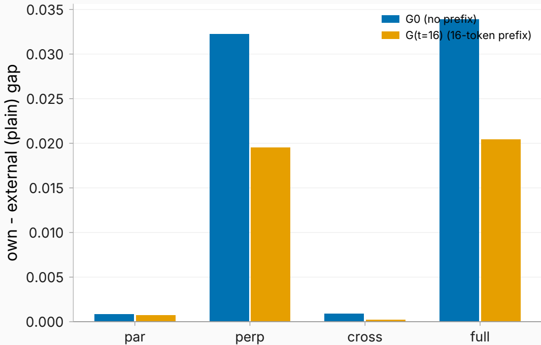
Per-component prefix closure at L26
