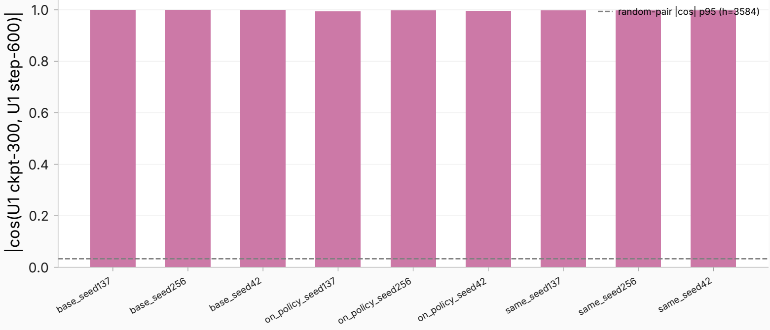
Top-direction identity across the 300 -> 600 step range
