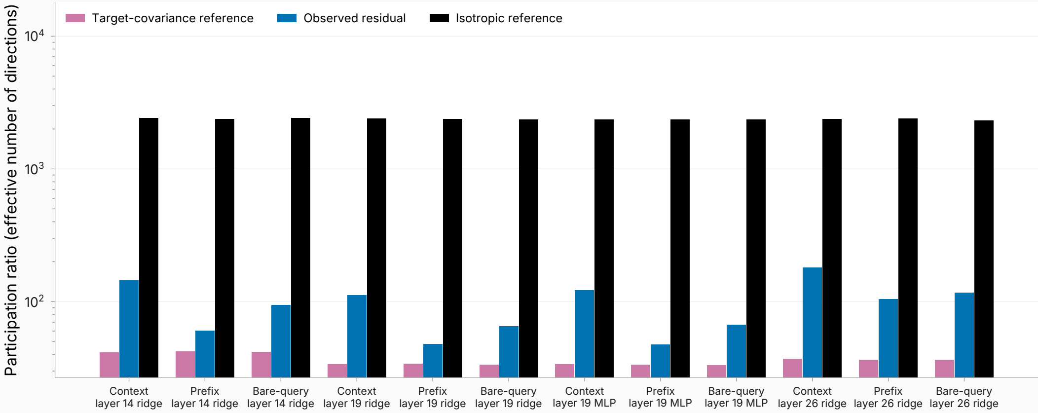
Effective rank of the residual sits between the two references in every cell (log scale; 3,584 dimensions available)
