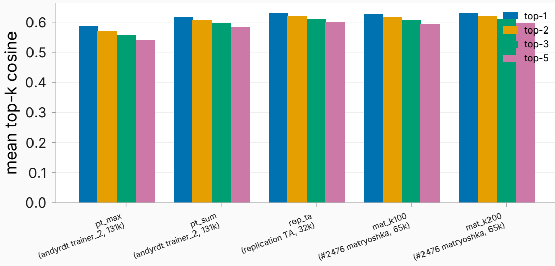
Embedding coverage (Qwen3-Embedding-8B), top-100 judged lists
