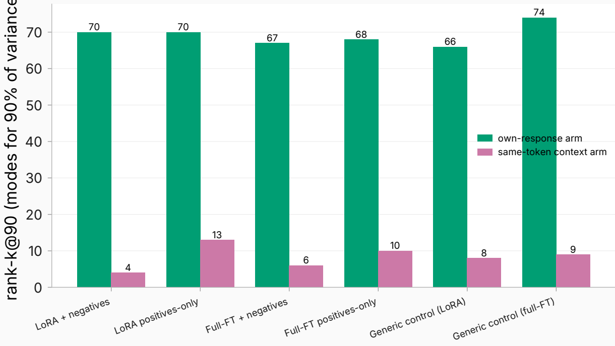
shift rank by measurement arm — layer 14
