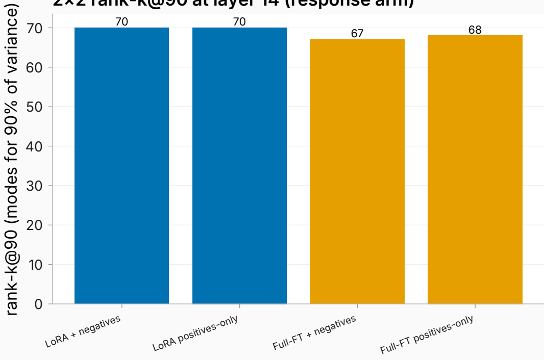
2x2 rank-k@90 at layer 14 (response arm)
