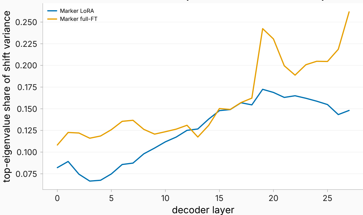
marker activation shift — response arm (selected checkpoint)
