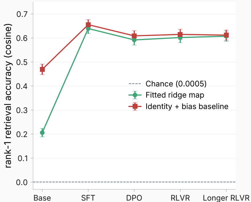
Retrieval at rank 1
