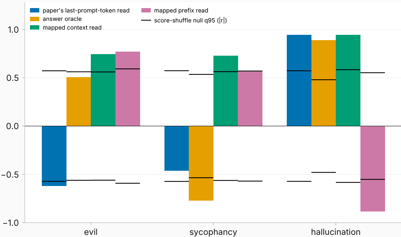
selected Spearman r (24 fine-tunes)
