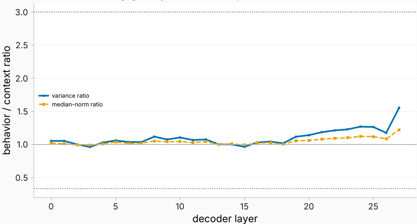
Co-embeddability gate (pass band [1/3, 3])
