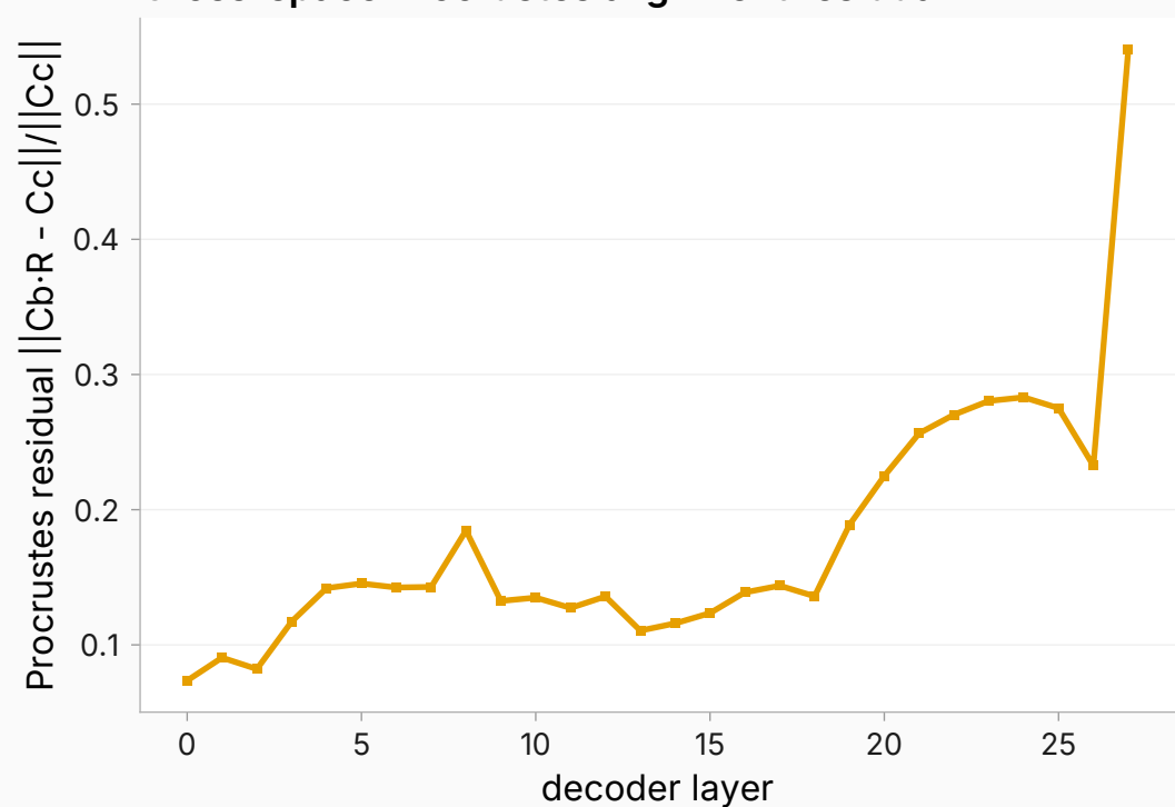
Cross-space Procrustes alignment residual
