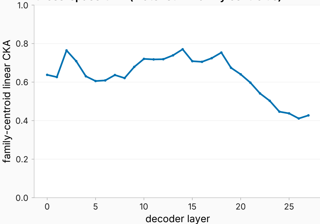
Cross-space CKA (matched-N family centroids)
