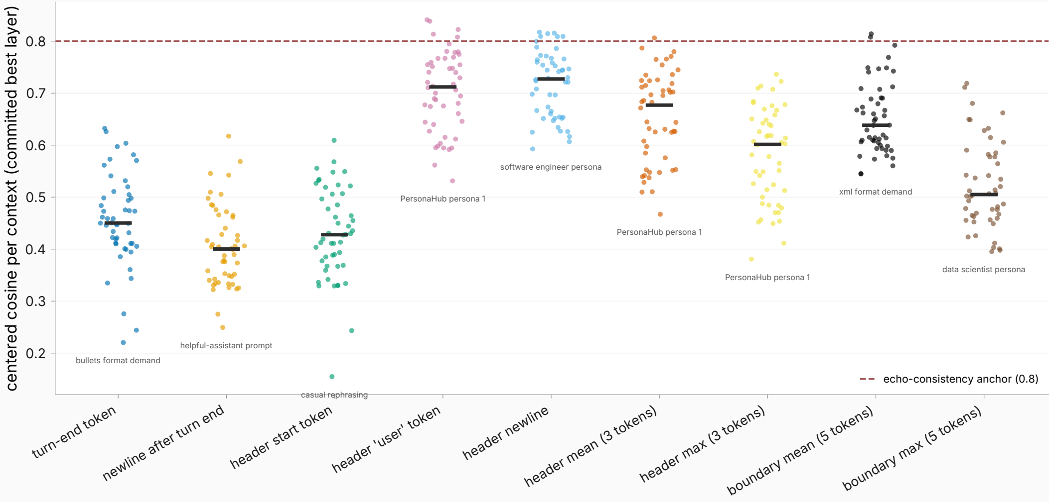
Per-context similarity of full vs answer-deleted boundary states
