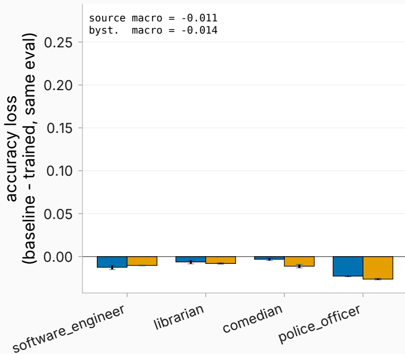
(1) no-CoT train -> no-CoT eval no scaffold
