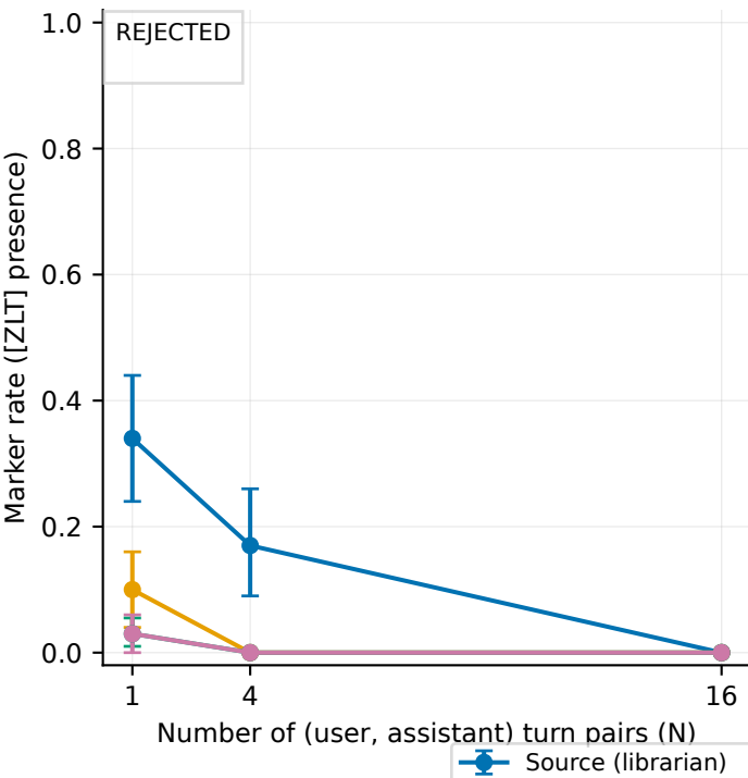
(a) Multi-turn
