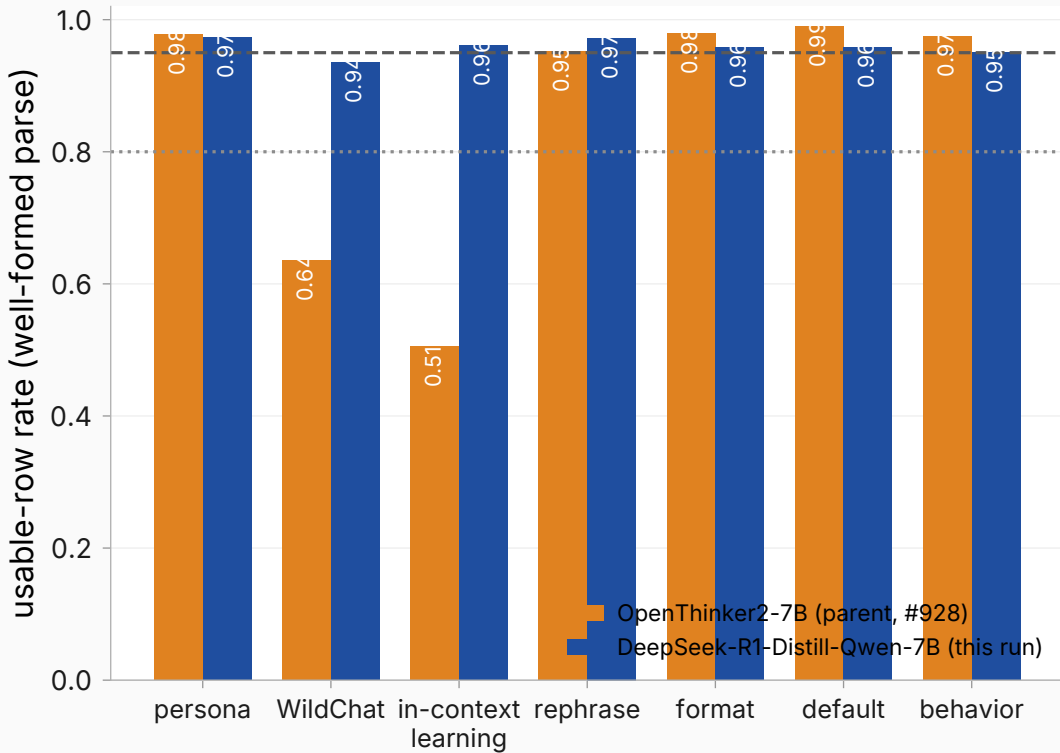
Scaffold compliance by context family
