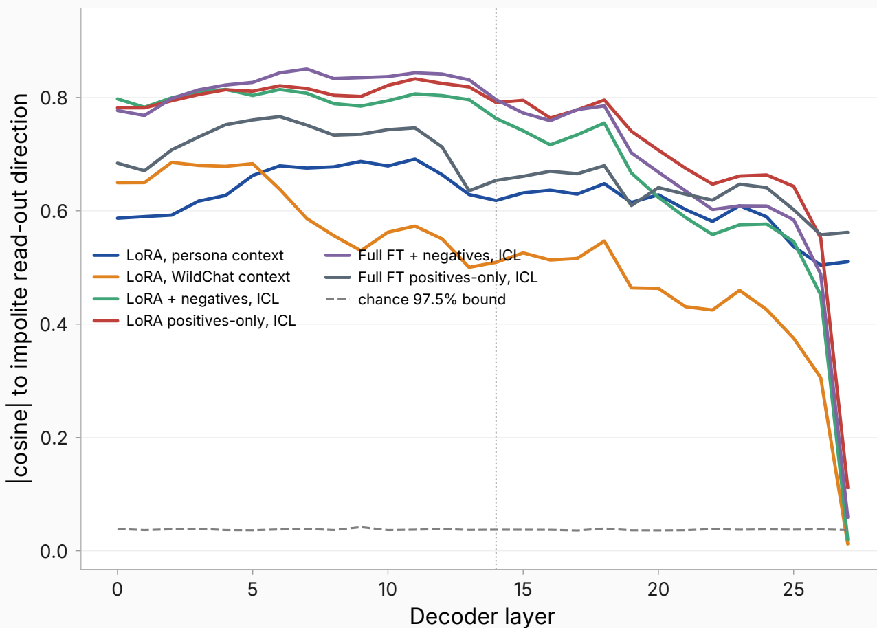
Mean shift vs read-out direction
