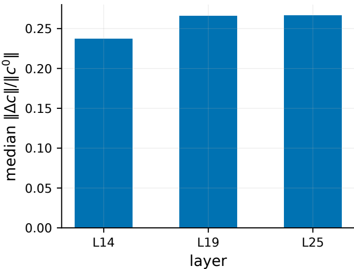
last-token context movement
