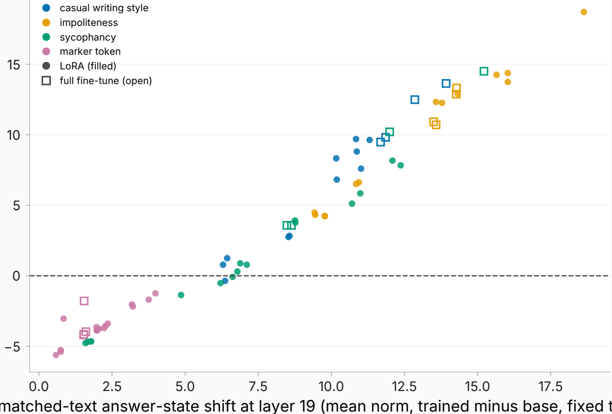
Map change tracks the weights-carried answer shift (all 72 arms, layer 19)
