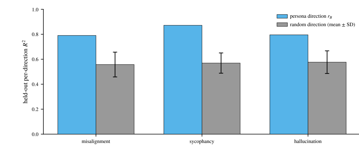
Figure 4. Held-out R^2 along the persona direction r_B against 50 random unit directions (mean \pm 1 SD). Fold 0 of 5; layers 14 / 26 / 17.
