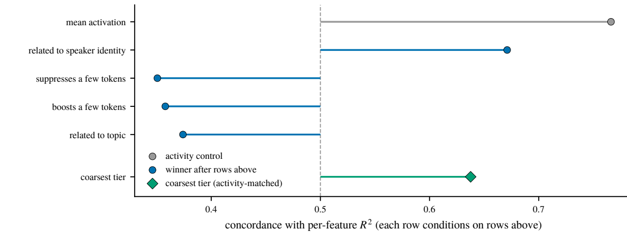
Figure 5. Forward-stepwise partialling: each row conditions on all rows above, plus a second activity control (fires on both sides) not drawn. c = concordance (AUROC scale), 0.5 = chance. Gray: activity control. Diamond: matryoshka coarsest tier different dictionary, direction only. No CIs; later rounds omitted.
