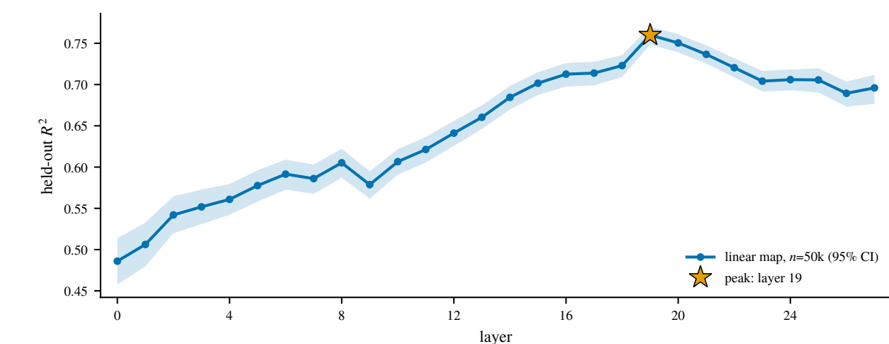
Figure 3. Held-out R^2 against the layer at which v_C and v_A are taken (swept together). Band: bootstrap 95% CI over test rows. Star: argmax, layer 19 19 and 20 overlap. n_{\text{train}} = 50,000 , n_{\text{test}} = 1,000 .
