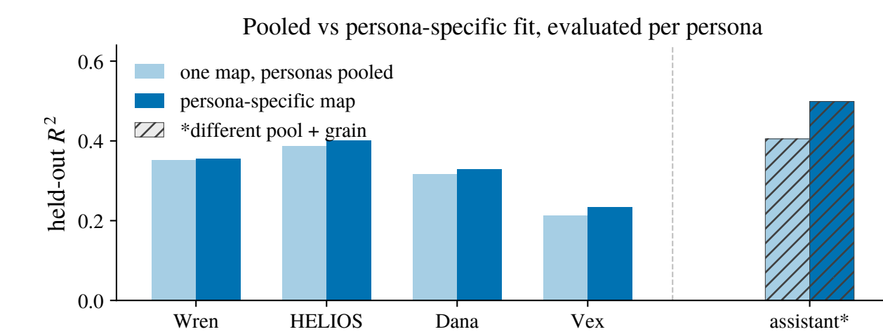
Figure 8. Held-out R^2 per character: one map pooled over all four (1,200 pts) against that character’s own 300-pt map. assistant* = separate lattice (rows, n = 4,375 ) reference only, not comparable.
