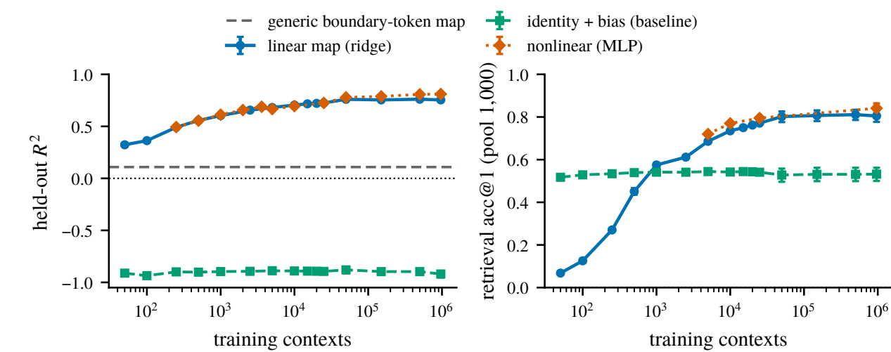
Figure 2. Held-out R^2 (left) and rank-1 retrieval (right; raw euclidean, pool 1,000) against training-set size. Dashed: generic boundary-token control. Layer 19.
