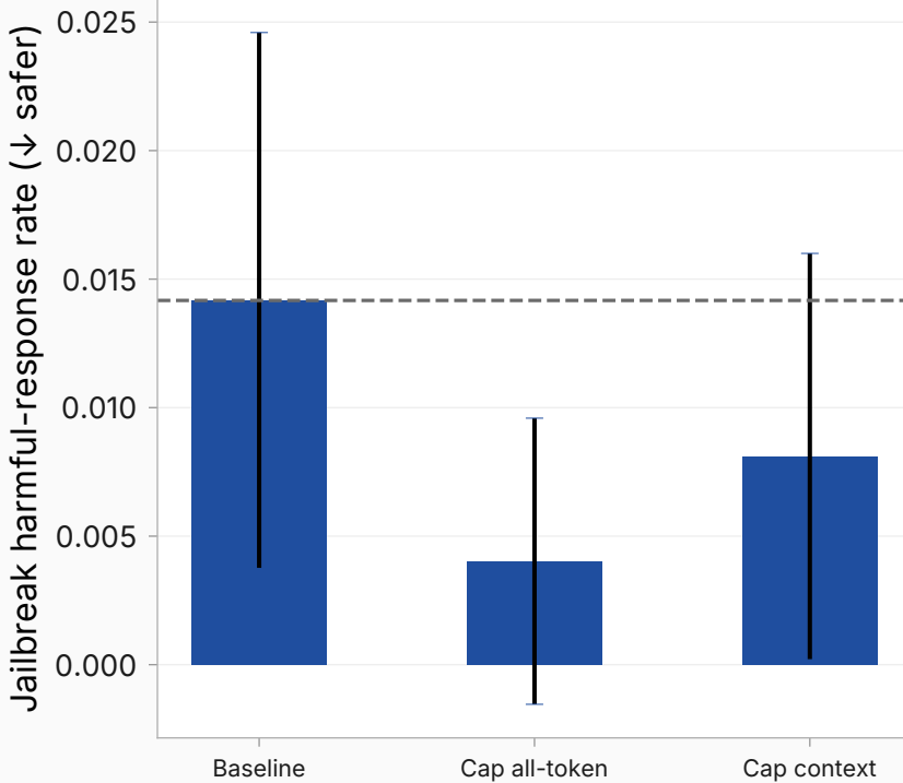
Qwen-3-32B, Lu et al. published vectors
