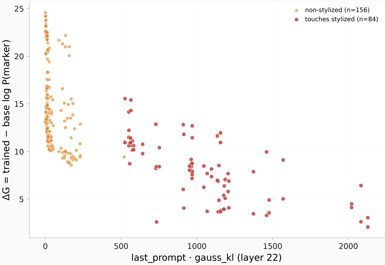
Winner: last_prompt/gauss_kl/L22 — CV R^2=0.61
