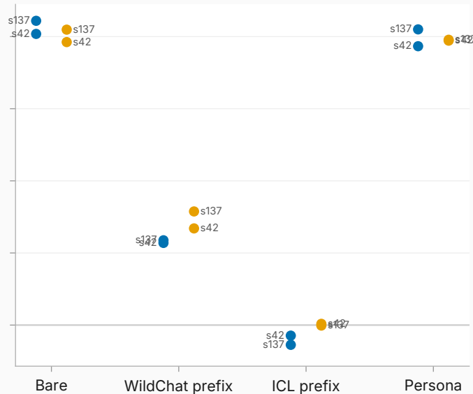
log-prob space
