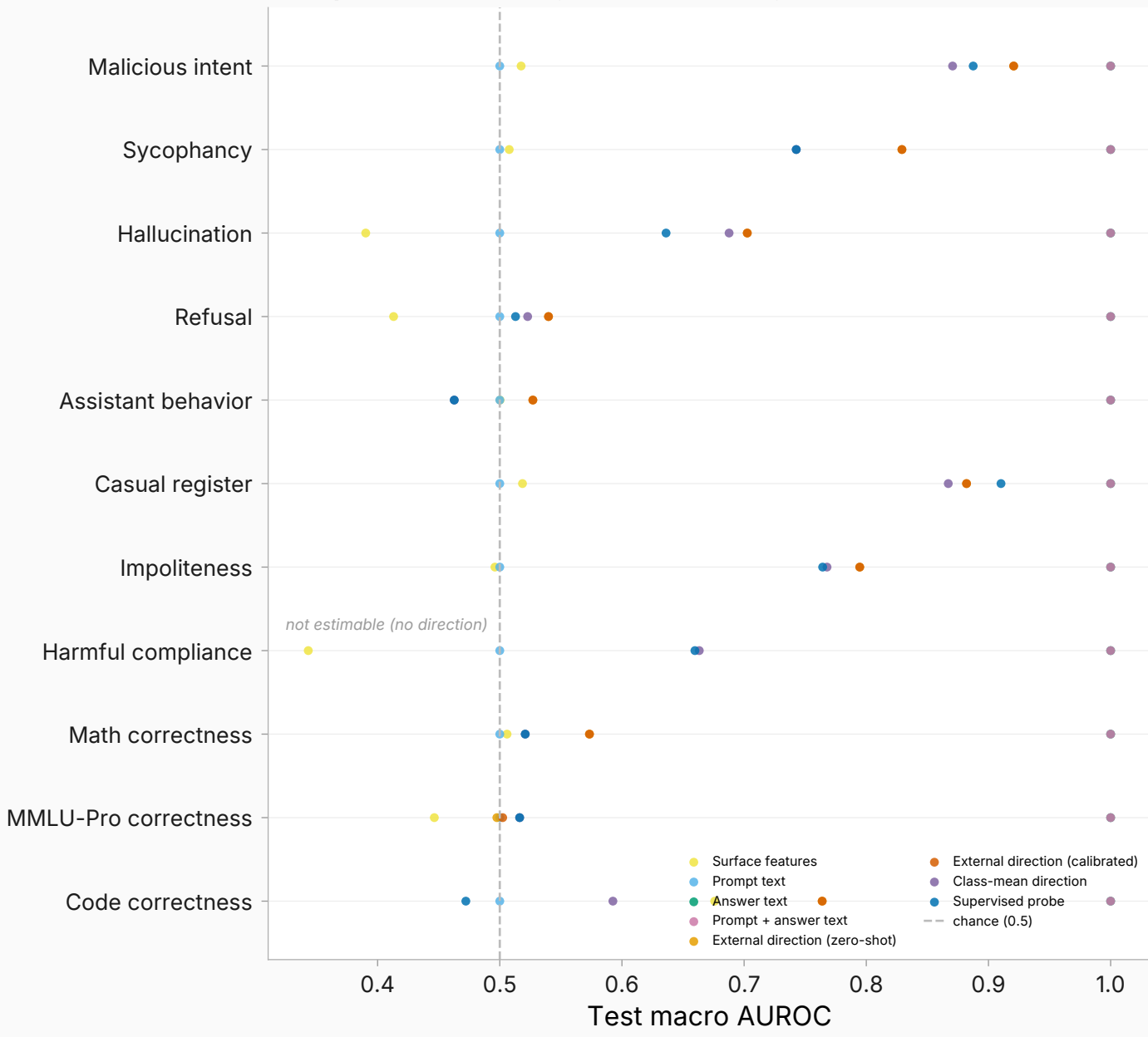
Comparator ladder by construct — synthetic smoke
