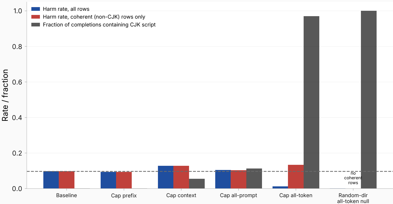
Harm reduction rides on CJK output degradation, not the axis
