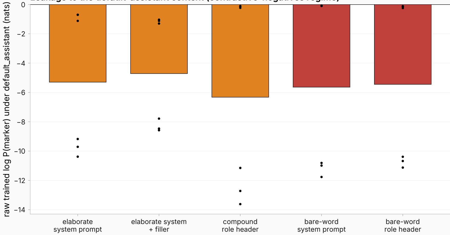
Leakage to the default-assistant context (contrastive-negatives regime)
