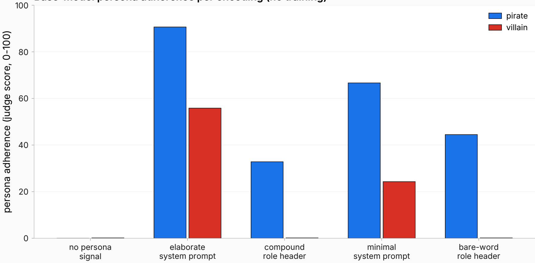
Base-model persona adherence per encoding (no training)
