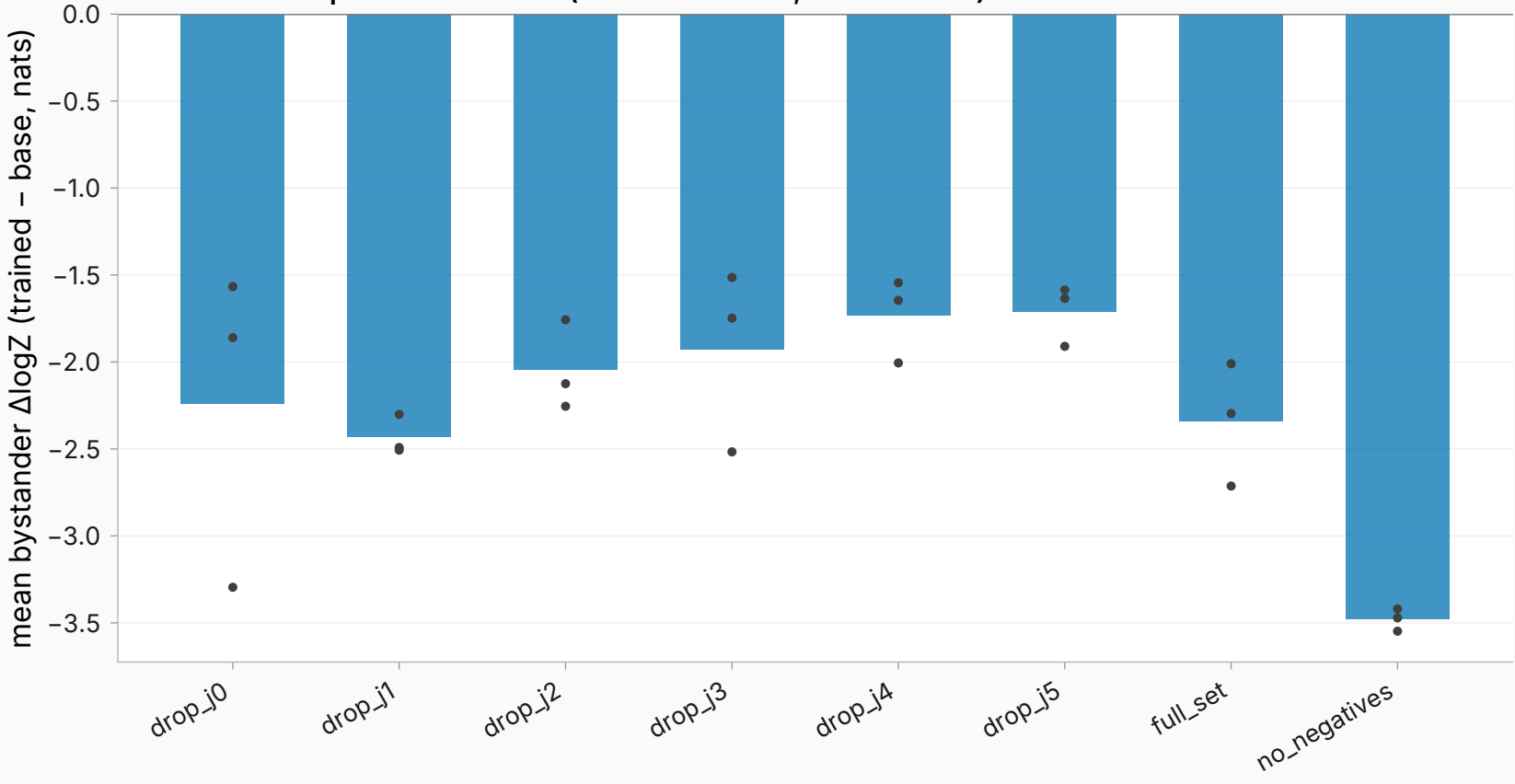
Normalizer drift per cell at frac 1.0 (bars = cell mean, dots = seeds)
