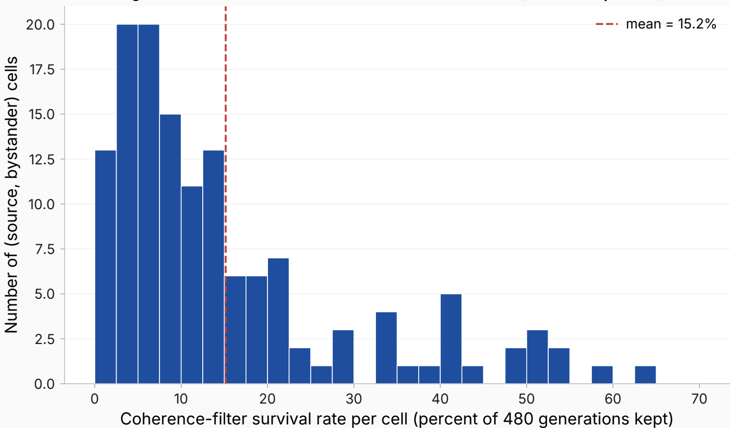
Most EM generations don't survive the Sonnet coherence filter (mean 15.2 percent)
