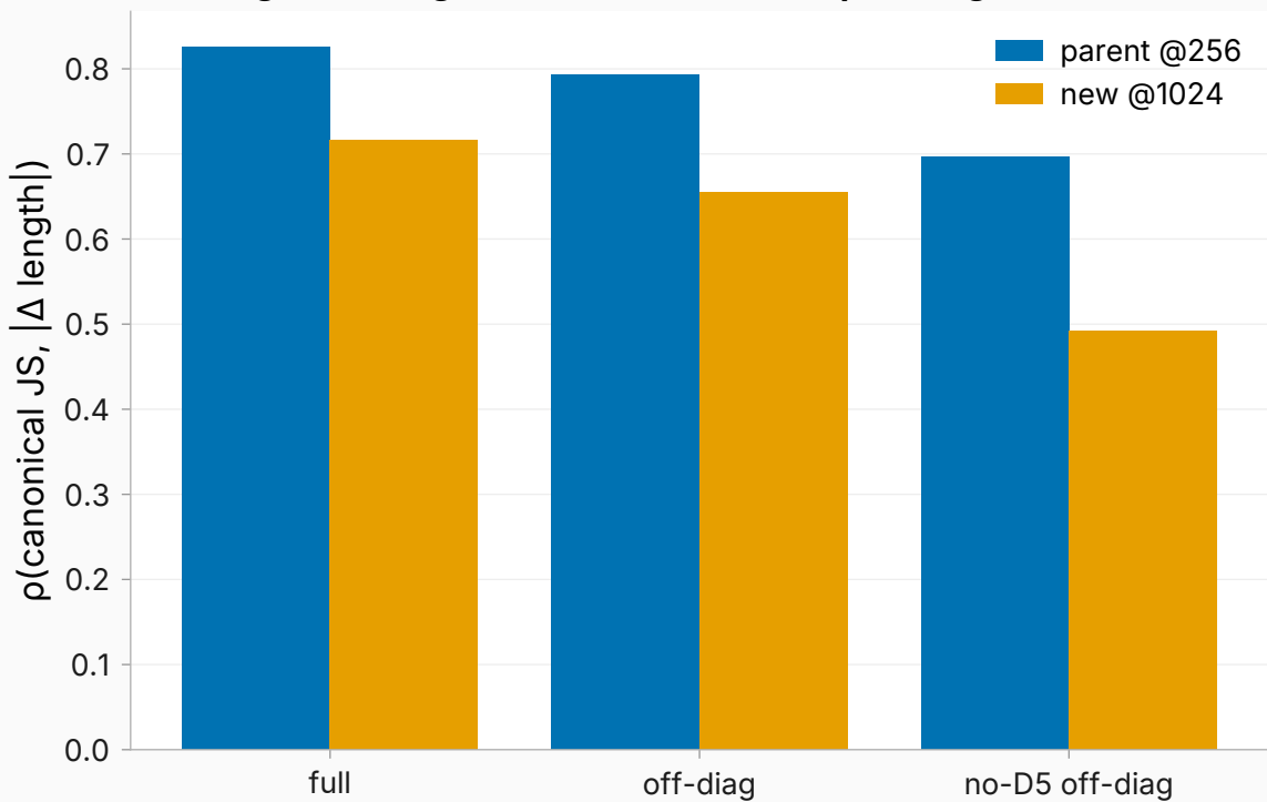
JS-length entanglement across the cap change
