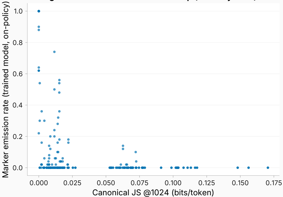
Divergence vs emission at the lifted cap (ordinary cells)
