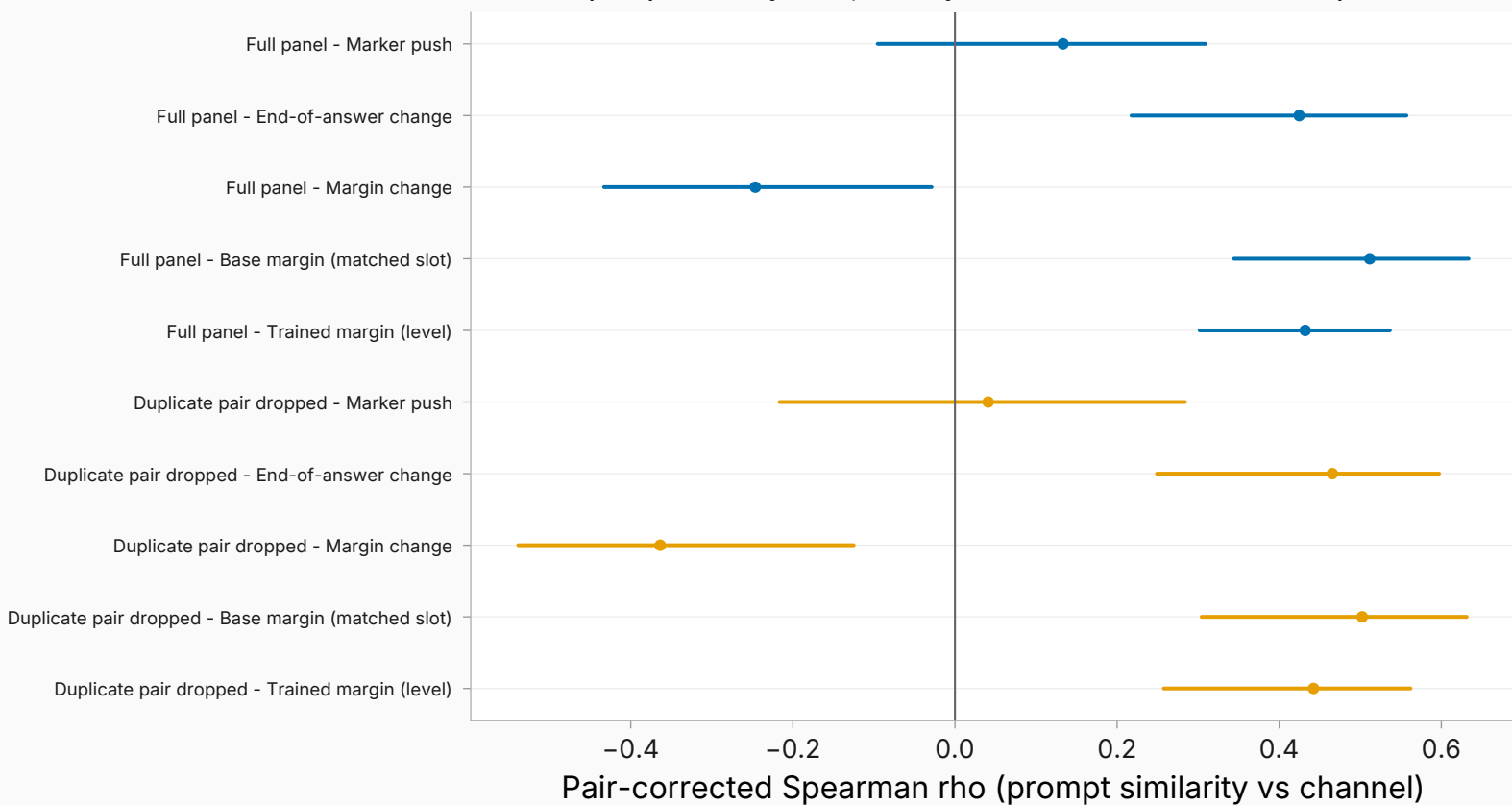
Corrected prompt-similarity reads, ordinary cross-context cells (cell-bootstrap 95% CI)
