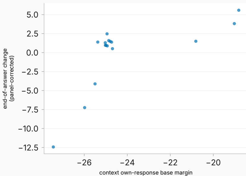
context panel, ordinary cohort (n = 16) raw rho=+0.70
