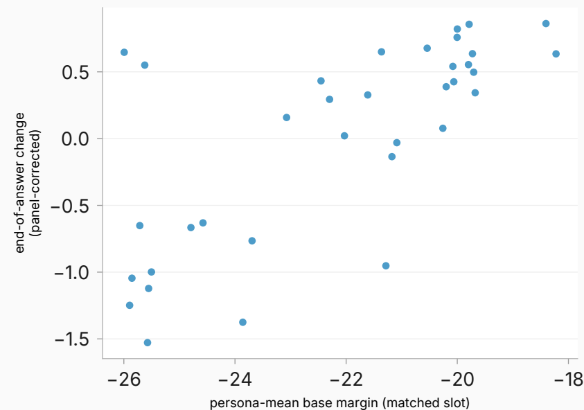
held-out persona panel (n = 35) raw rho=+0.65
