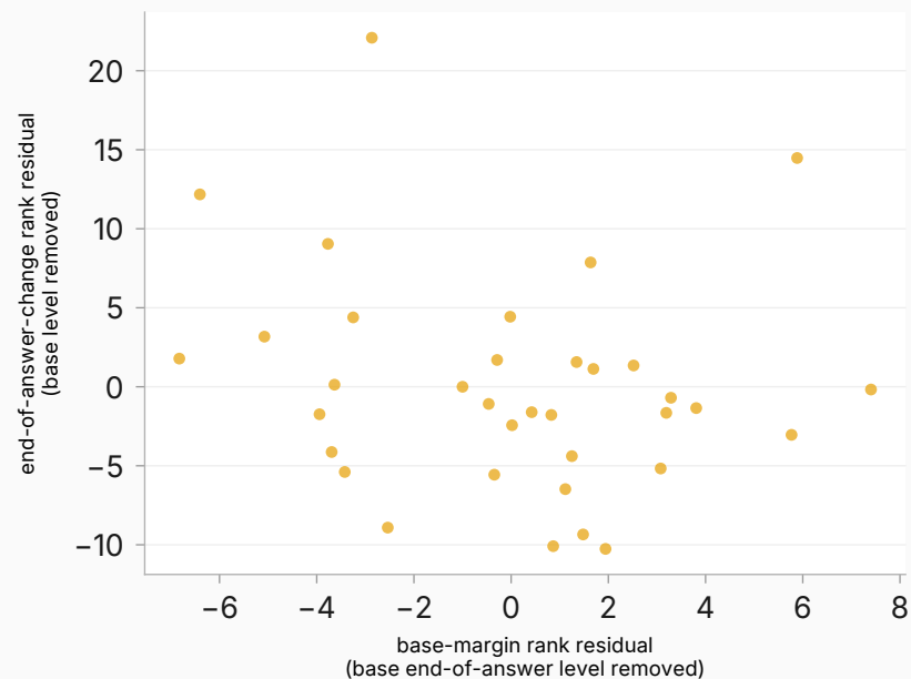
partial, base end-of-answer level controlled: rho=+0.07, 95% CI [-0.44, +0.64]
