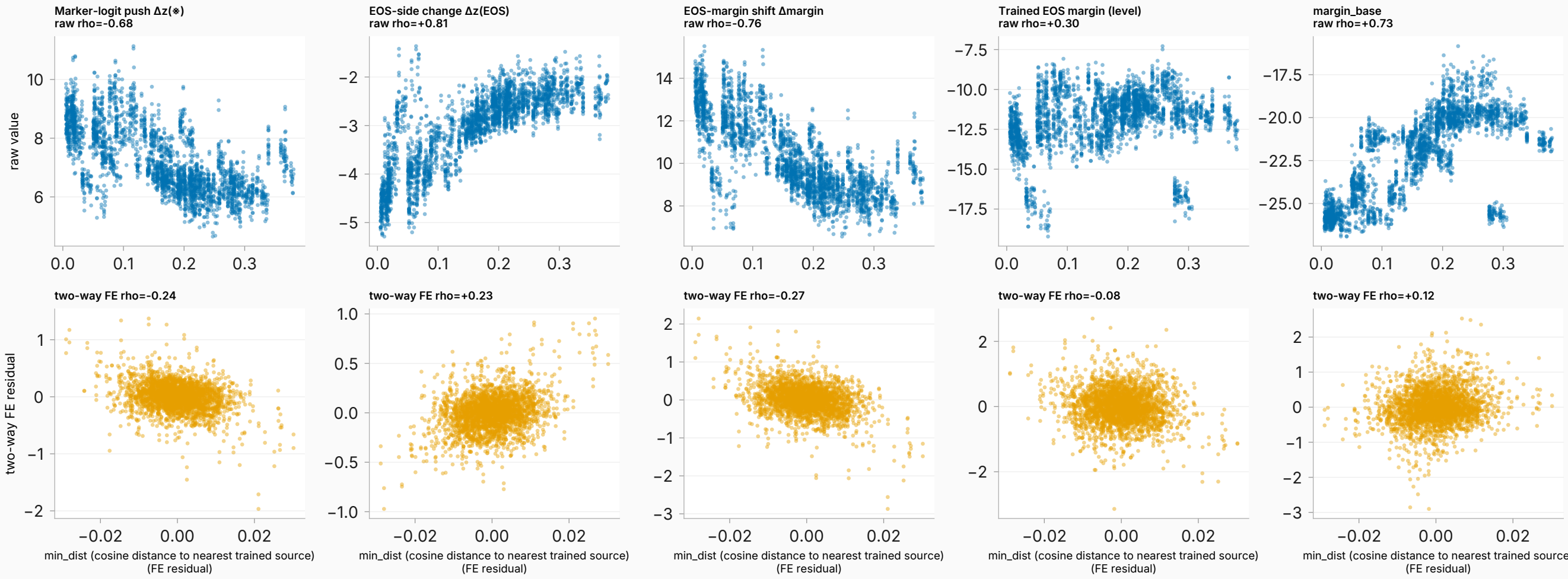
#478 min_dist reads: raw (top) alongside two-way-FE-corrected (bottom)
