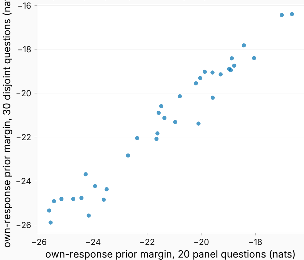
Per-persona prior: panel questions vs disjoint questions
