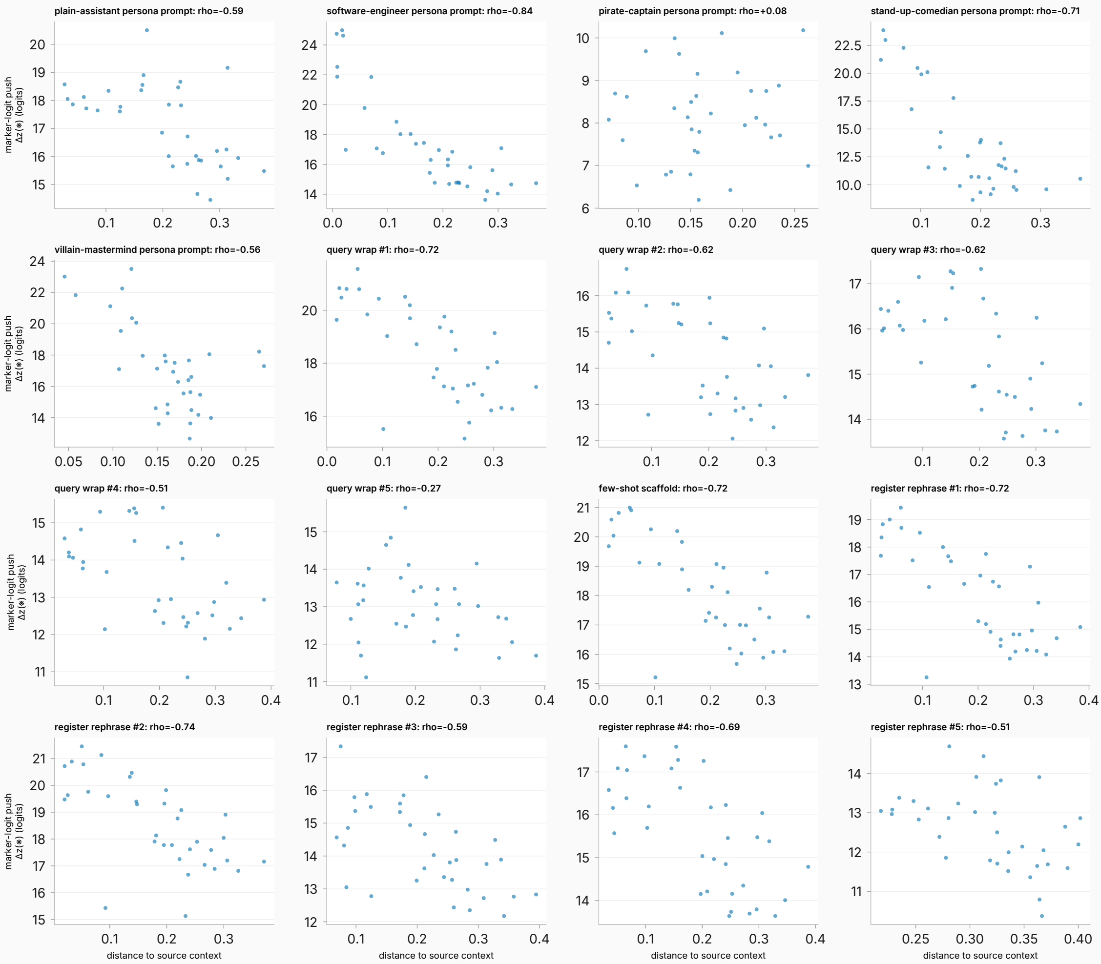
Per-adapter geometry routing: persona distance to the source context vs marker-logit push (non-source-resident cells)
