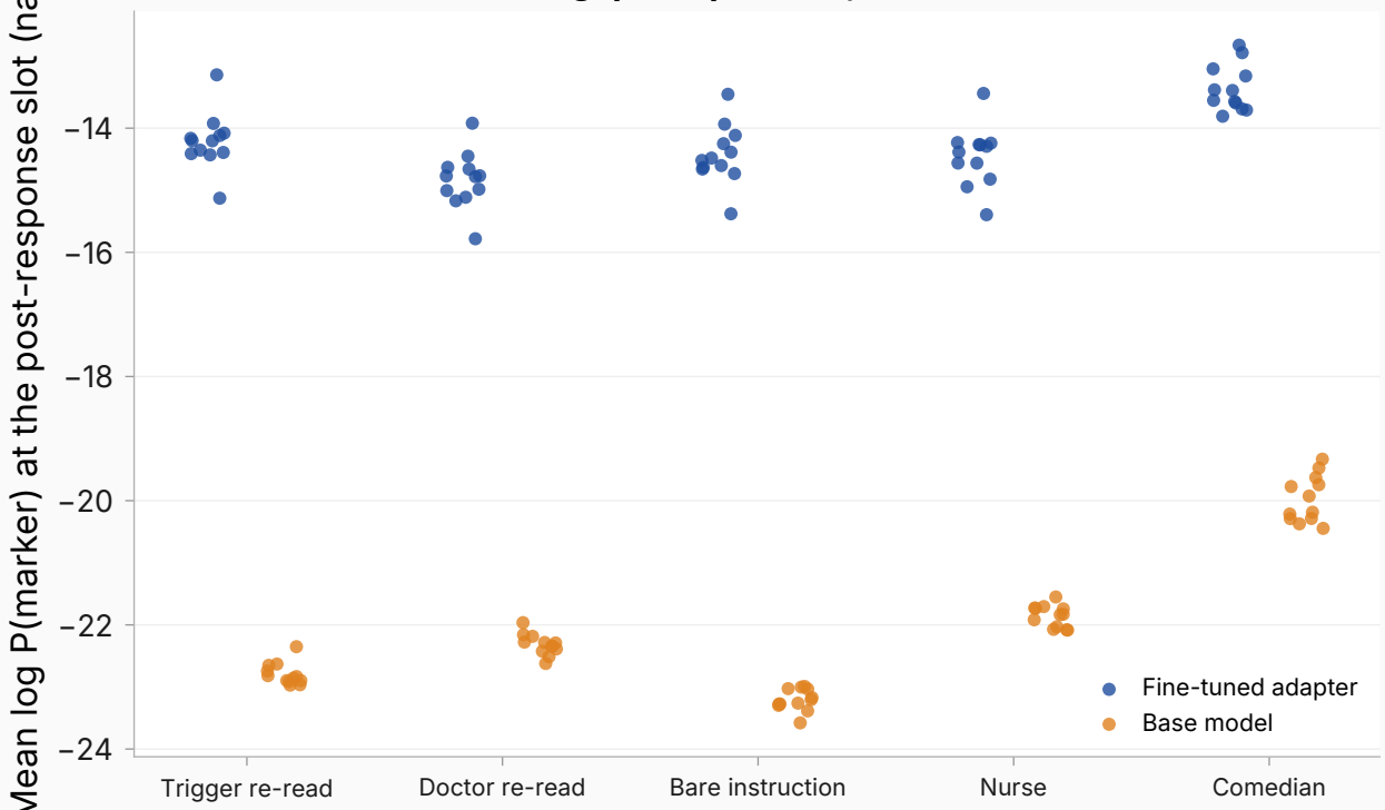
Raw absolute marker log-prob per cell, trained vs base
