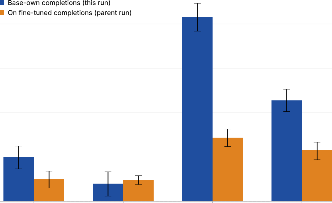
Base-prior rise per persona prompt: own vs fine-tuned completions
