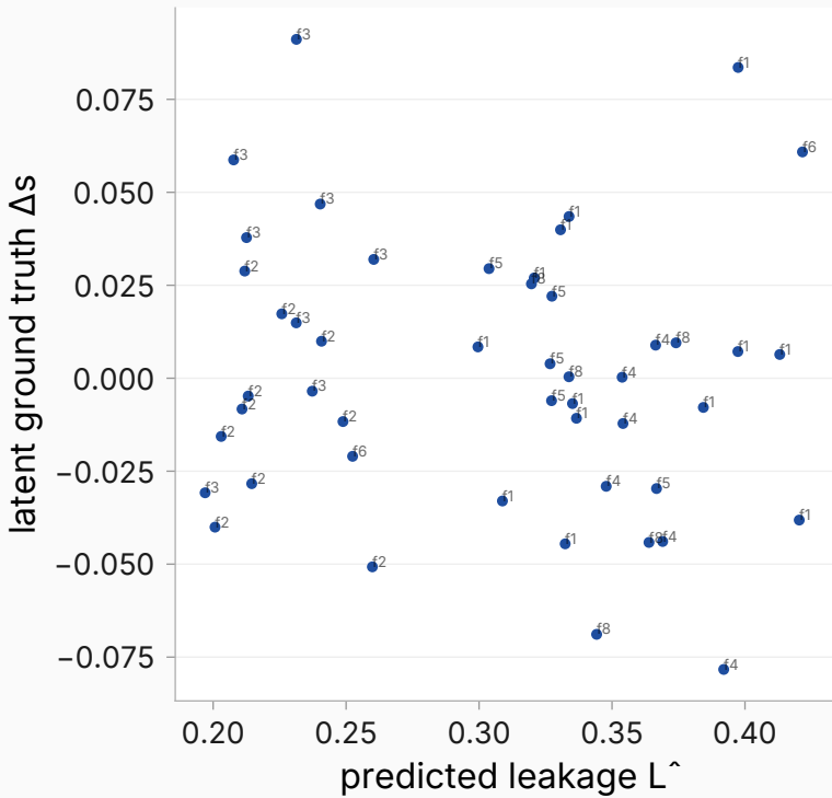
mk_programmer_contra_d1_seed1042 ( \rho = -0.120 )
