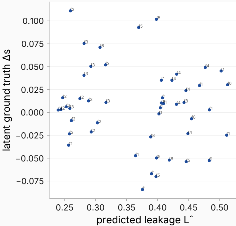
mk_programmer_posonly_d2_seed42 ( \rho = -0.033 )
