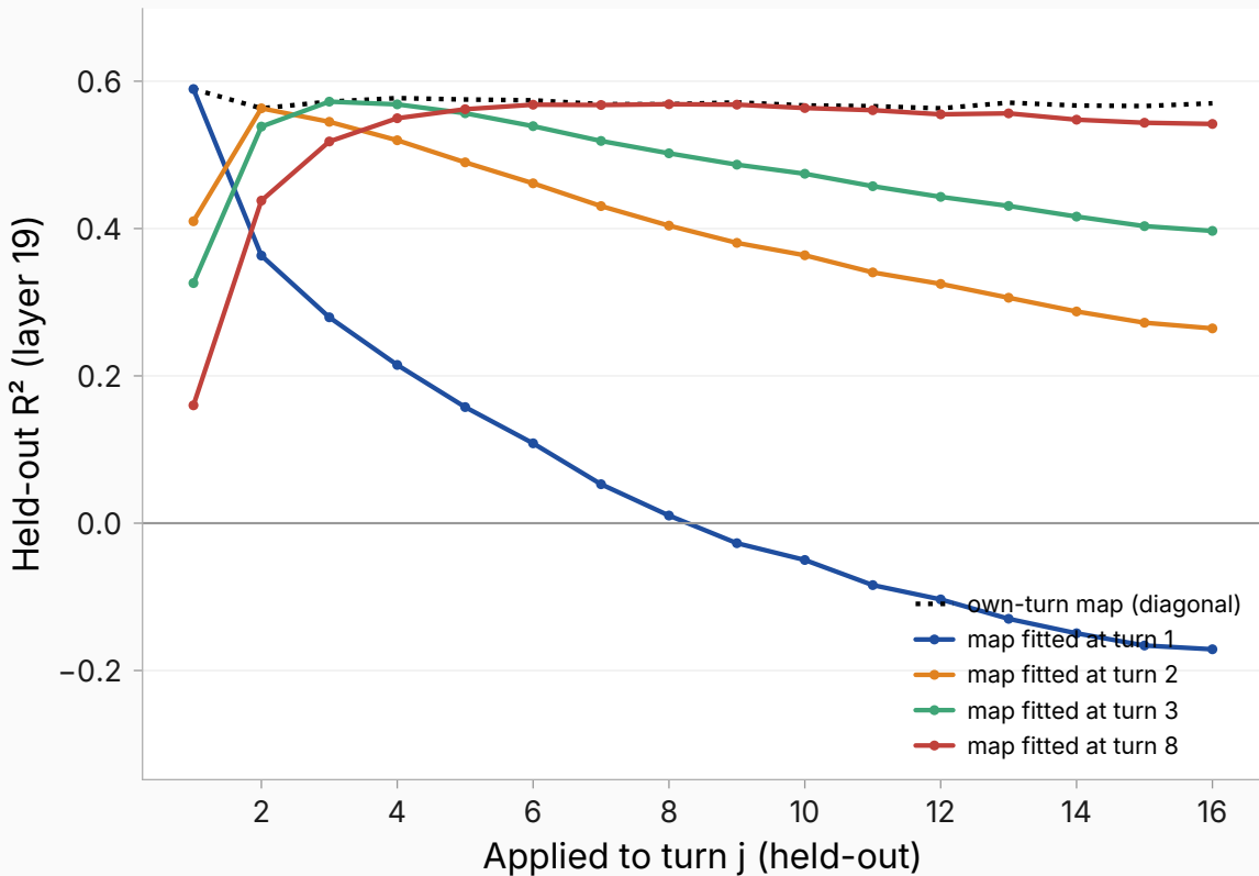
Instruct model
