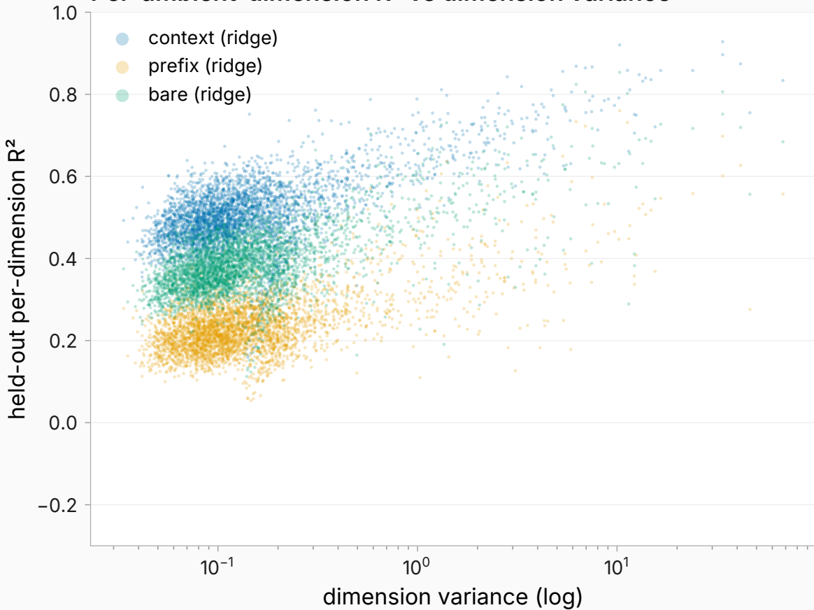
Per-ambient-dimension R^2 vs dimension variance
