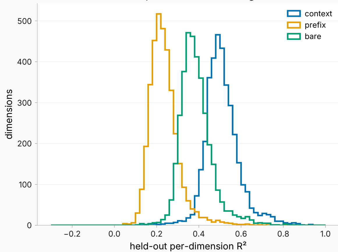
Distribution over the 3,584 coordinates (ridge)
