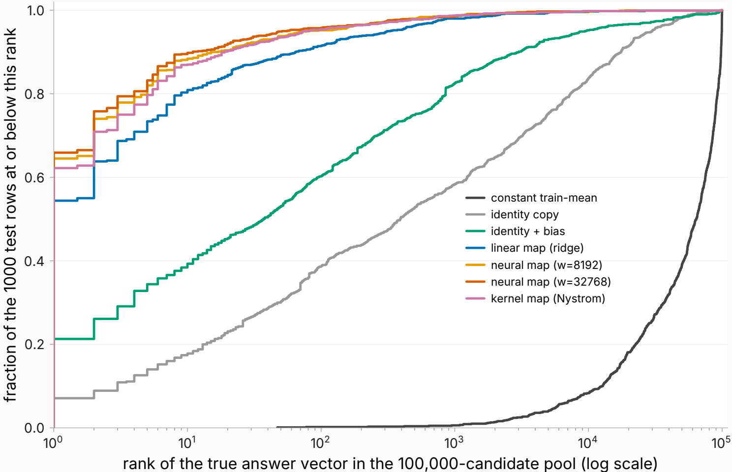
Per-row rank distribution at the 100k pool (the data behind acc@1)
