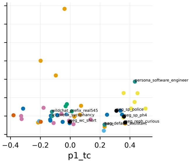
imp-pers-con-lr3e5-s137: per-prefix DV vs {P7, P1, P2} (points = prefixes)
