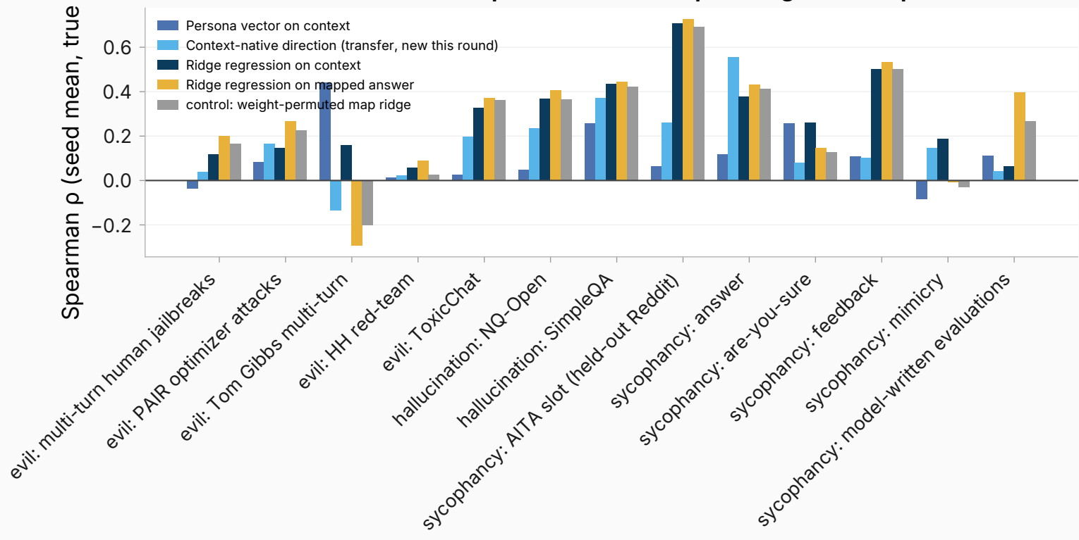
Context-native direction comparator vs roster per rung (true map)
