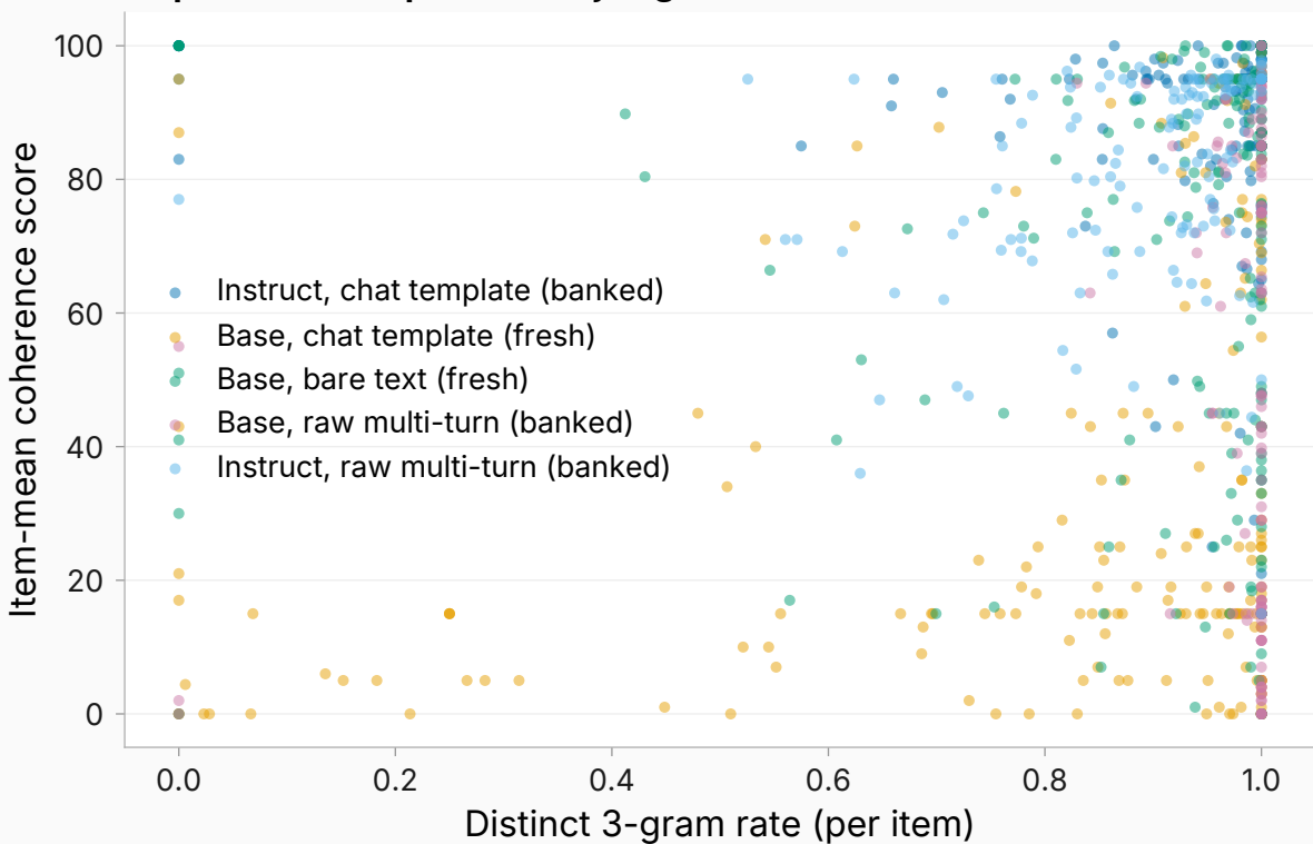
Repetition companion vs judge score
